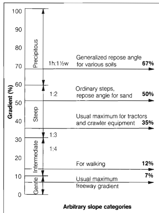
Figure 3. Slope categories (gentle, intermediate, steep, and precipitous) are based on use limitations and repose angles of some materials but have arbitrary ranges.
