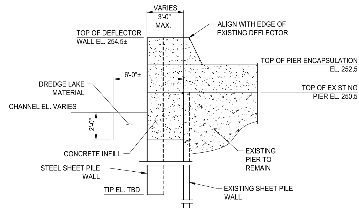
SECTION - NEW DEFLECTOR WALL
