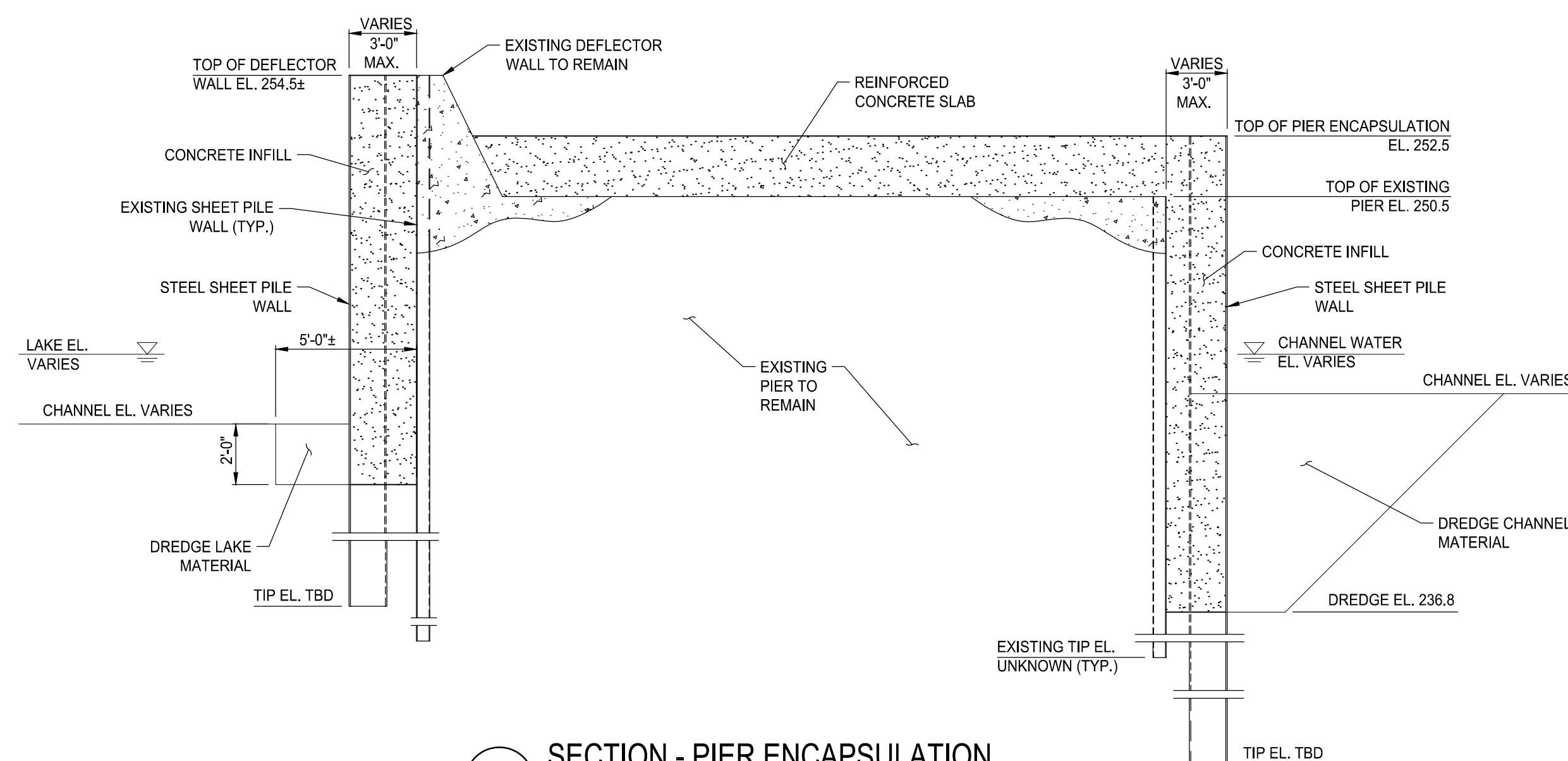
SECTION - PIER ENCAPSULATION
